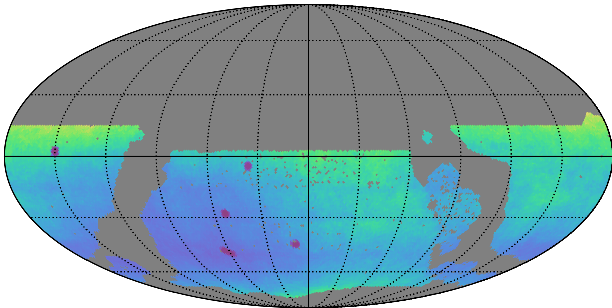
too_5_4v3.4_10yrs WFD: Parallax Uncert @ 24.0
