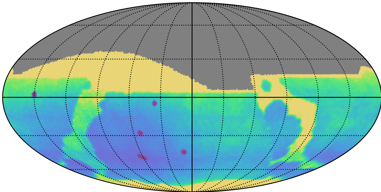
too_5_4v3.4_10yrs All sky: Parallax Uncert @ 24.0
