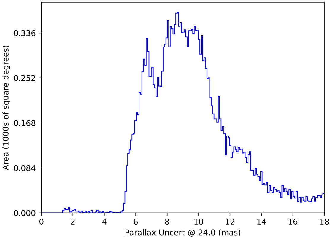
too_5_4v3.4_10yrs All sky: Parallax Uncert @ 24.0
