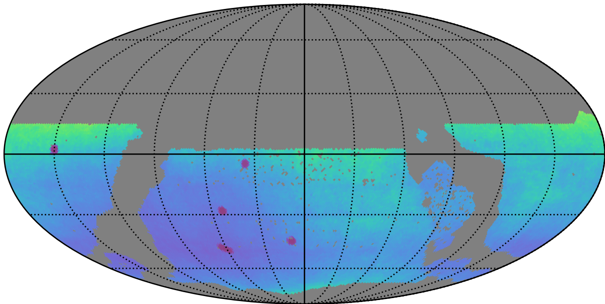
too_5_4v3.4_10yrs WFD: Parallax Uncert @ 22.4
