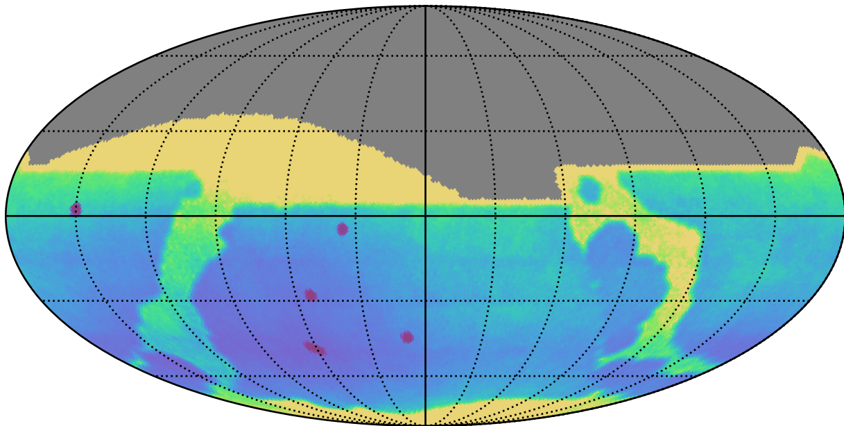
too_5_4v3.4_10yrs All sky: Parallax Uncert @ 22.4
