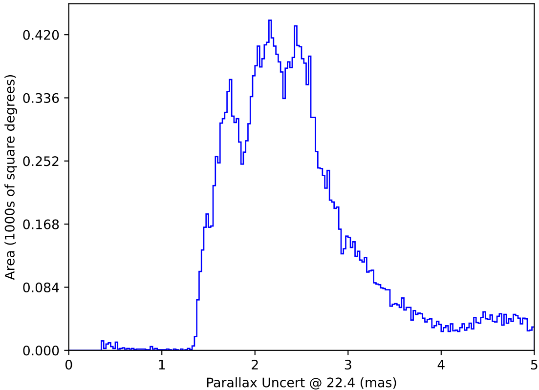
too_5_4v3.4_10yrs All sky: Parallax Uncert @ 22.4
