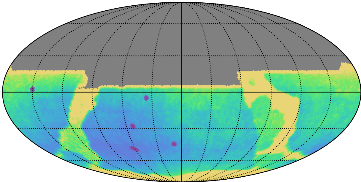
too_5_4v3.4_10yrs All sky y band only: Parallax Uncert @ 21.3
