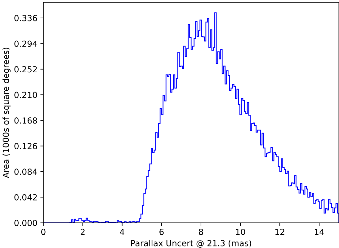
too_5_4v3.4_10yrs All sky y band only: Parallax Uncert @ 21.3
