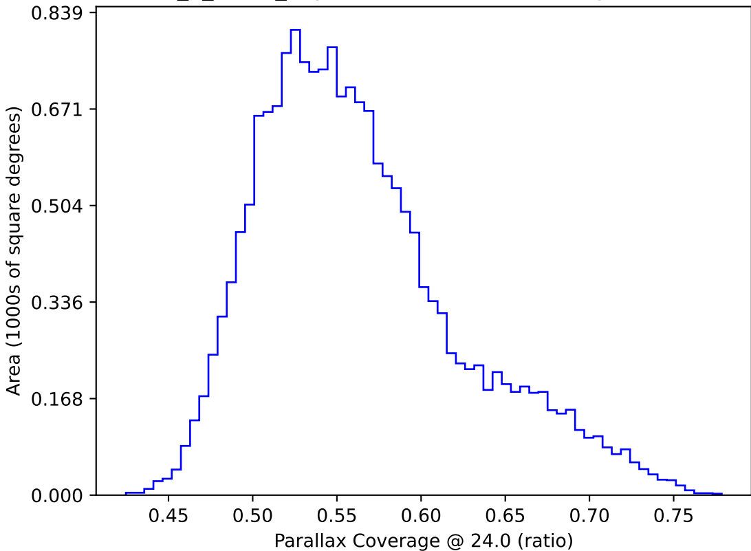
too_5_4v3.4_10yrs WFD: Parallax Coverage @ 24.0
