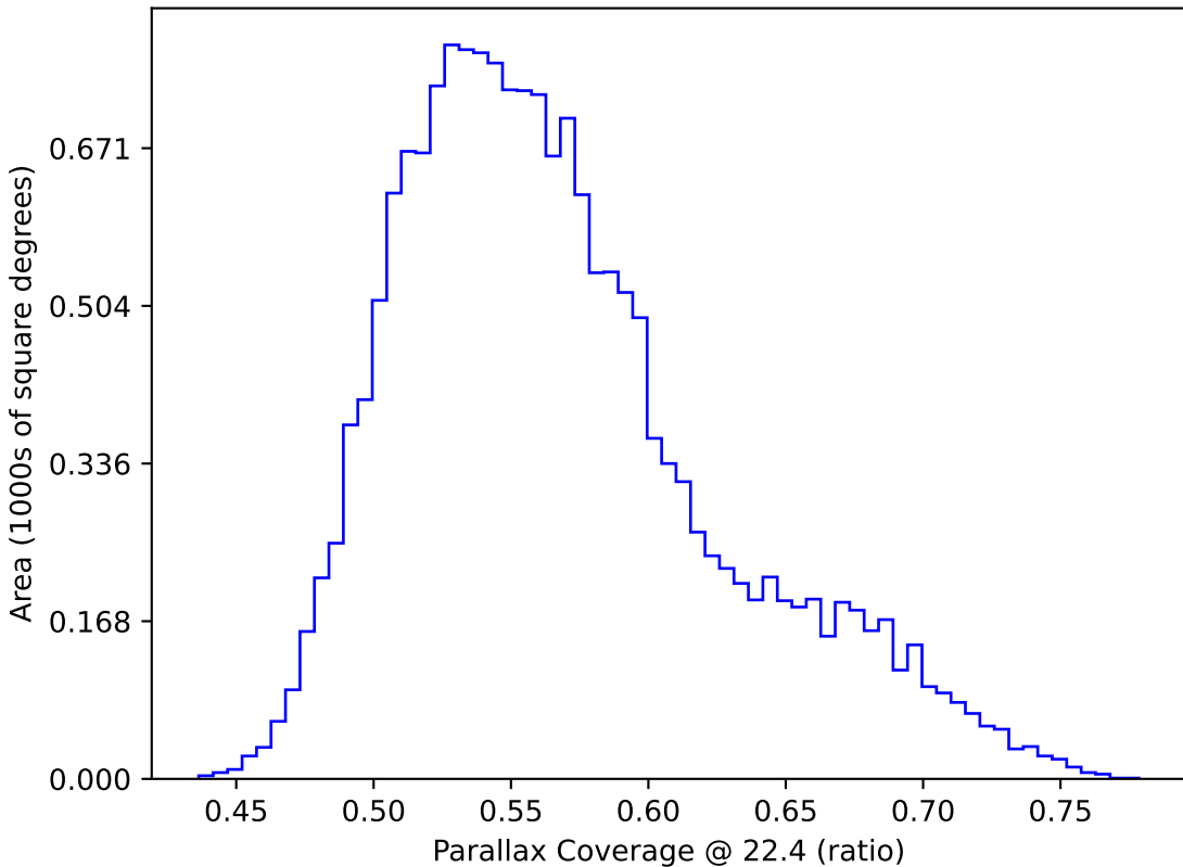
too_5_4v3.4_10yrs WFD: Parallax Coverage @ 22.4
