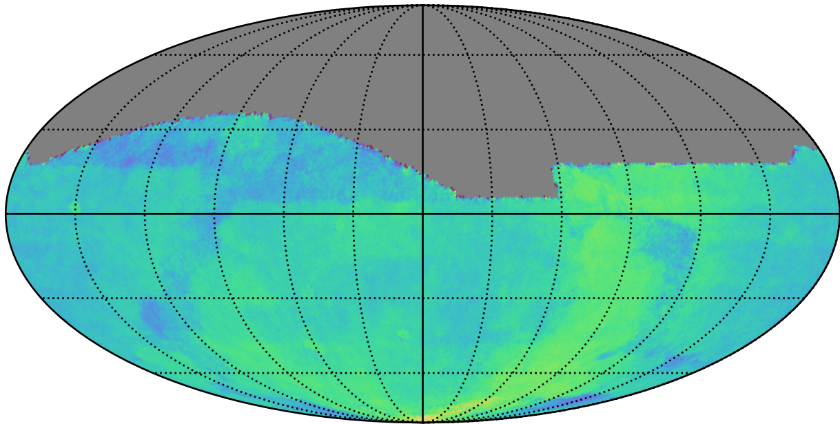
too_5_4v3.4_10yrs All sky: Parallax Coverage @ 22.4
