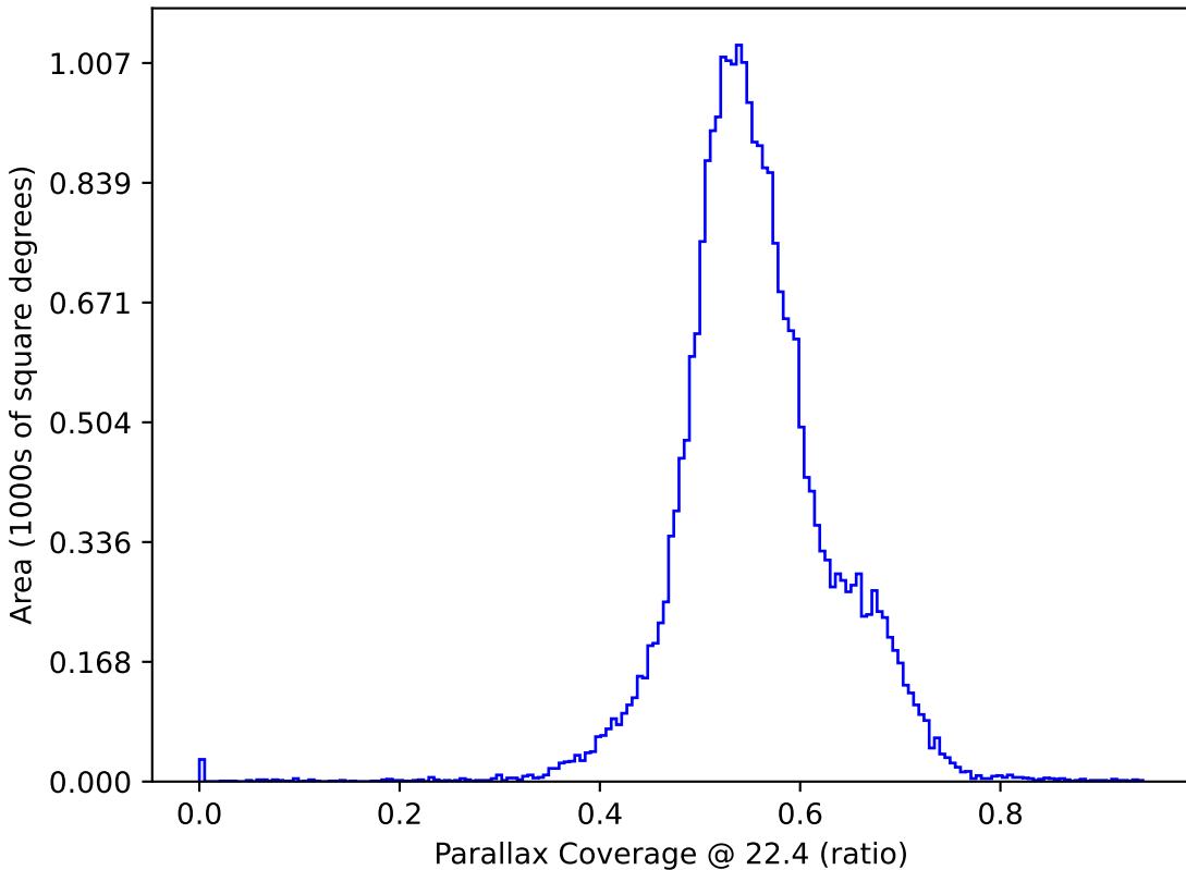
too_5_4v3.4_10yrs All sky: Parallax Coverage @ 22.4
