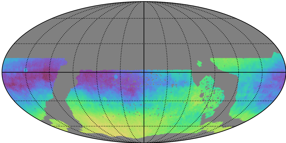
too_5_4v3.4_10yrs WFD: Parallax-DCR degeneracy @ 24.0
