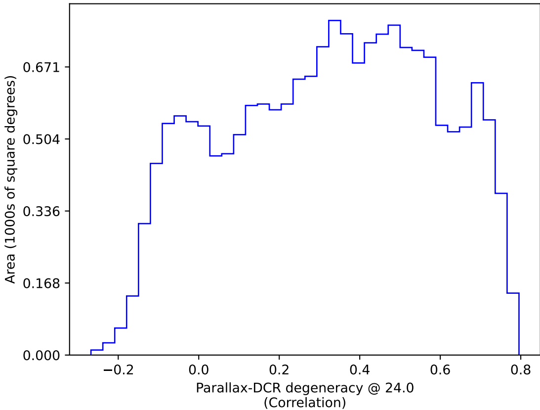
too_5_4v3.4_10yrs WFD: Parallax-DCR degeneracy @ 24.0
