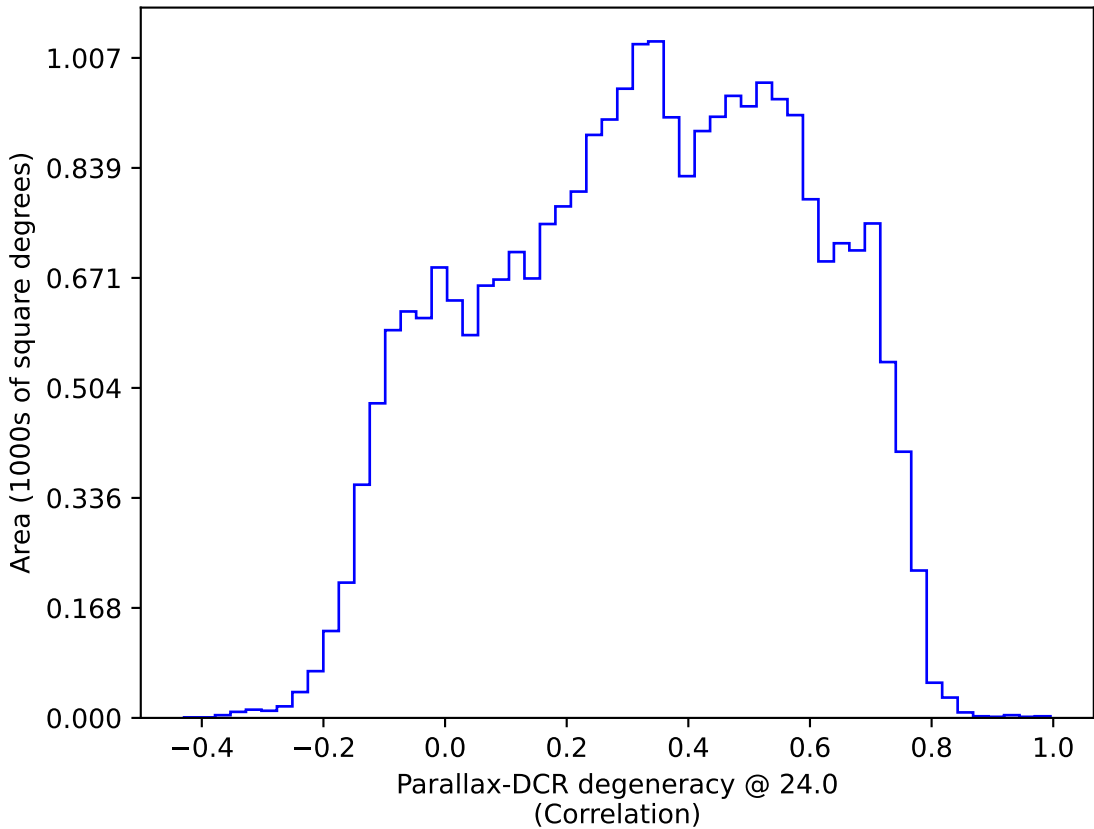
too_5_4v3.4_10yrs All sky: Parallax-DCR degeneracy @ 24.0
