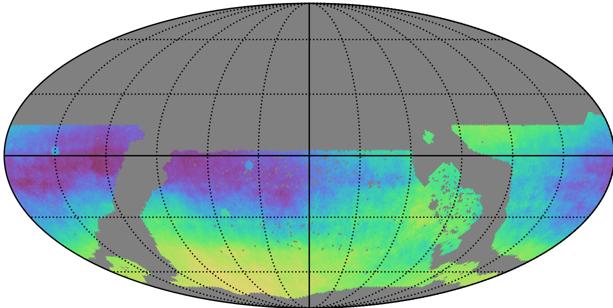
too_5_4v3.4_10yrs WFD: Parallax-DCR degeneracy @ 22.4
