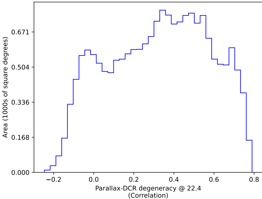
too_5_4v3.4_10yrs WFD: Parallax-DCR degeneracy @ 22.4
