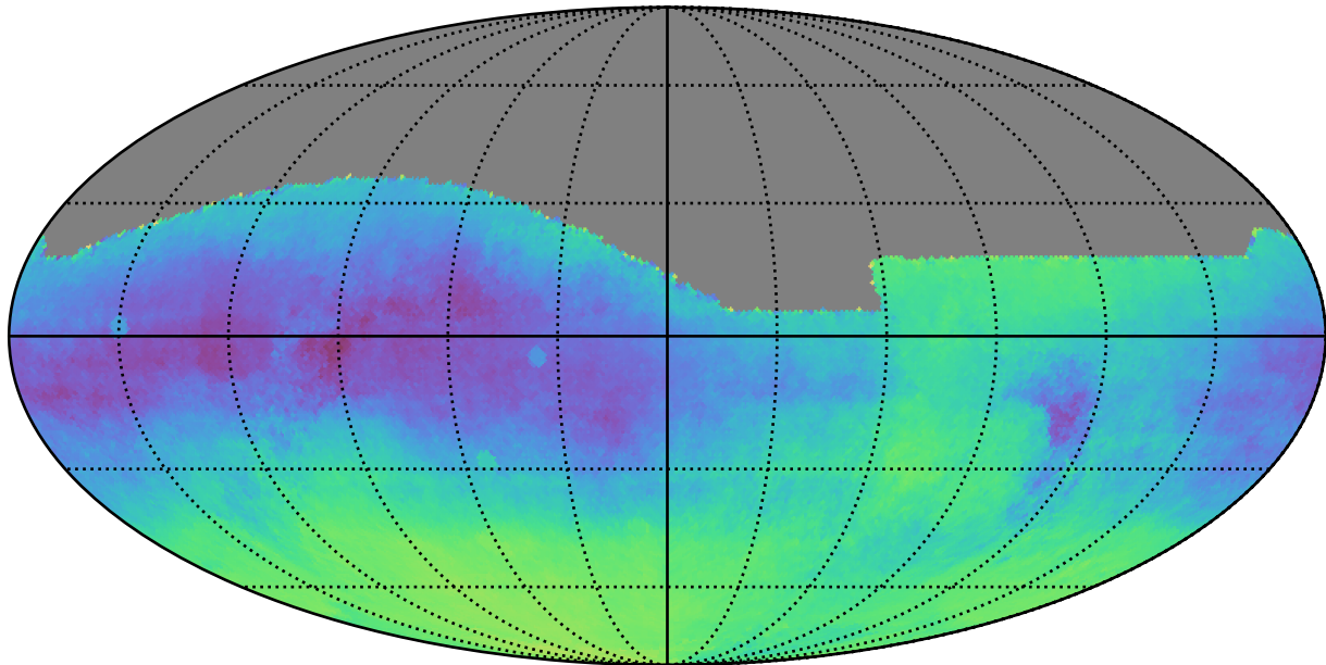
too_5_4v3.4_10yrs All sky: Parallax-DCR degeneracy @ 22.4
