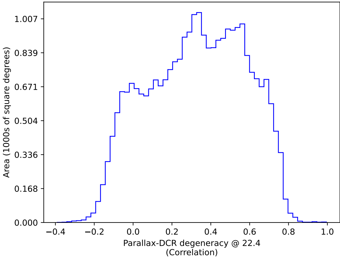
too_5_4v3.4_10yrs All sky: Parallax-DCR degeneracy @ 22.4
