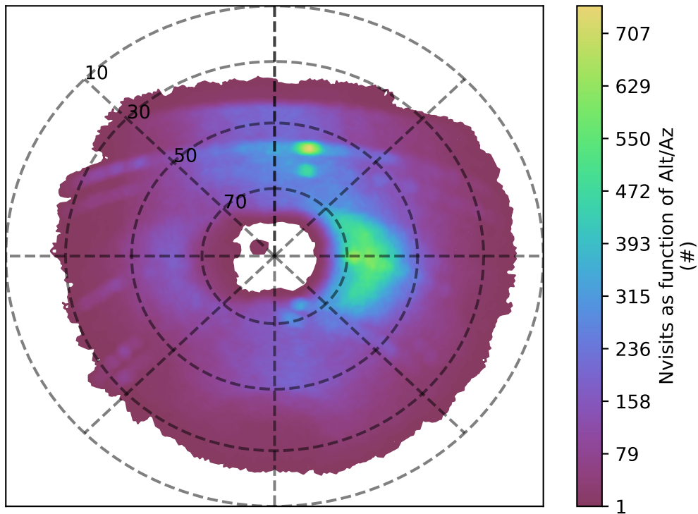
too_5_4v3.4_10yrs u band: Nvisits as function of Alt/Az
