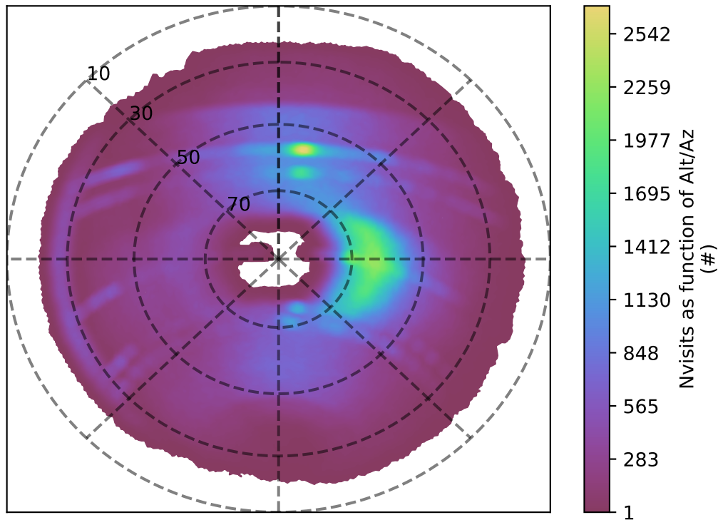
too_5_4v3.4_10yrs r band: Nvisits as function of Alt/Az
