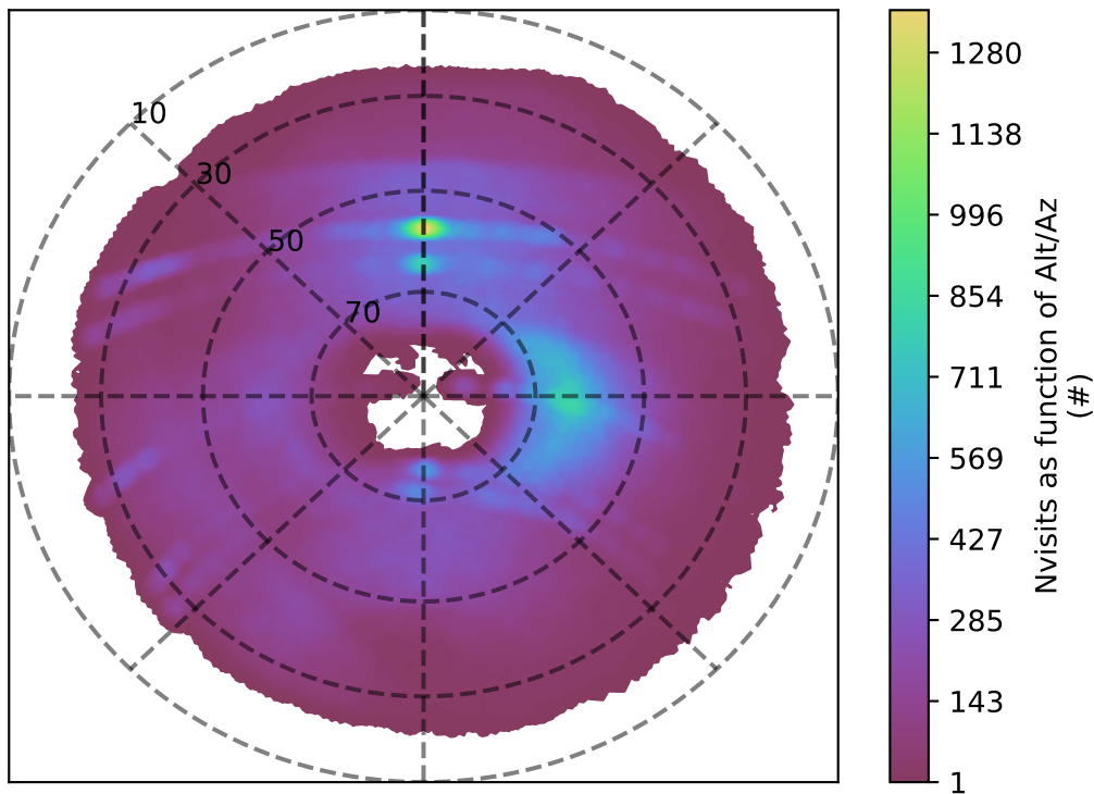
too_5_4v3.4_10yrs g band: Nvisits as function of Alt/Az
