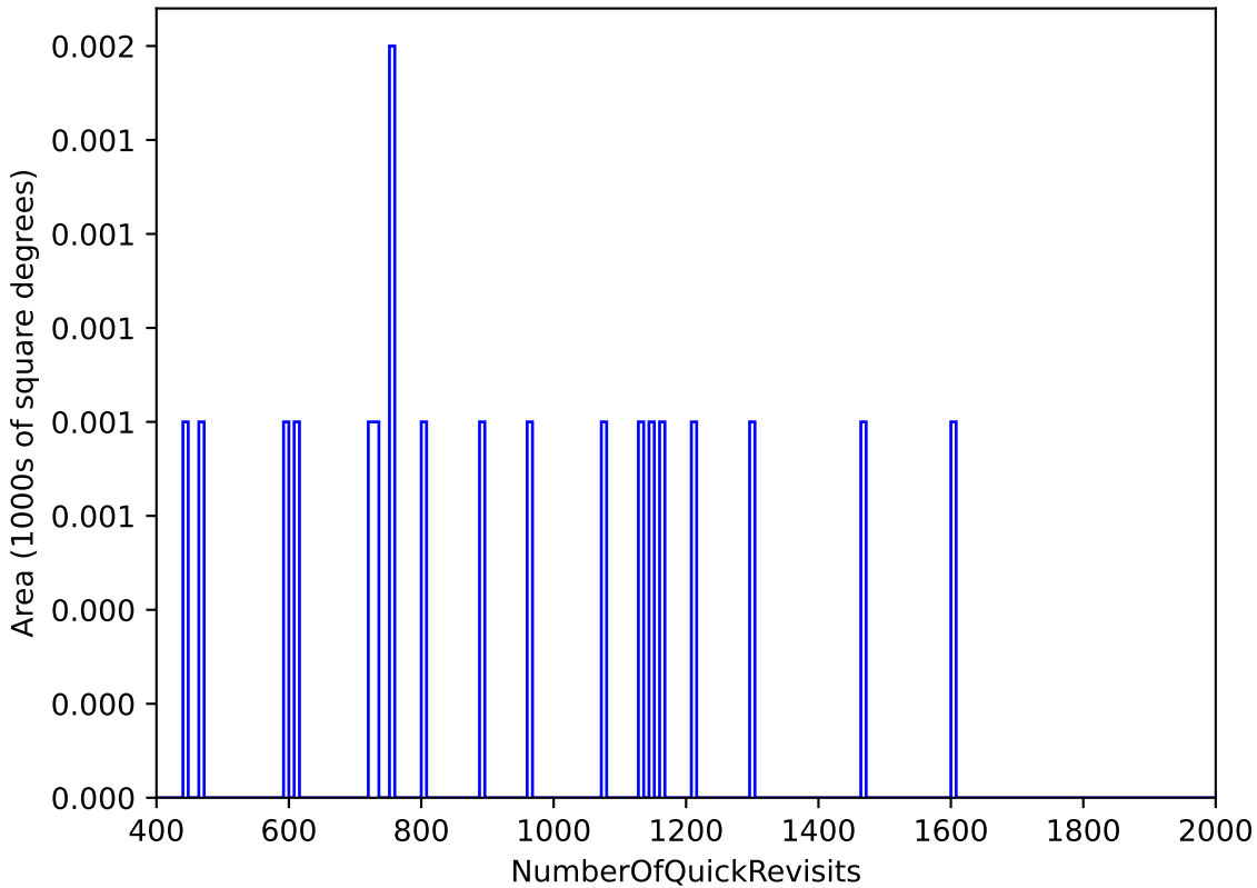
too_5_4v3.4_10yrs All sky: NumberOfQuickRevisits
