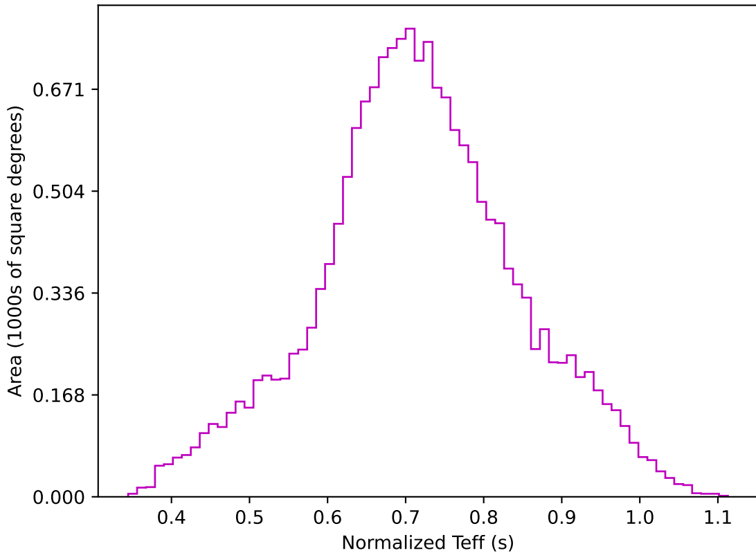
too_5_4v3.4_10yrs WFD z band: Normalized Teff
