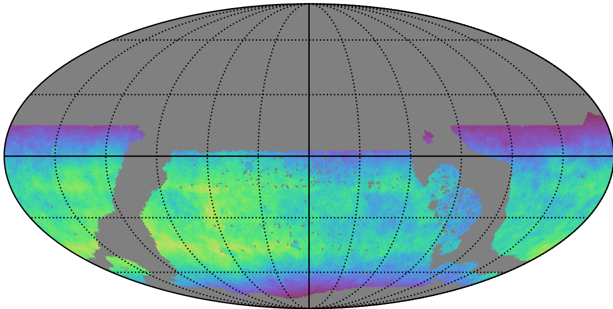
too_5_4v3.4_10yrs WFD y band: Normalized Teff
