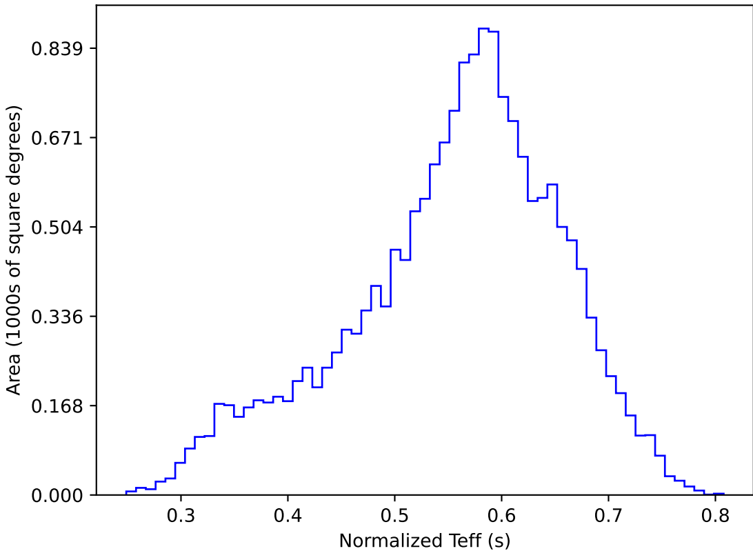
too_5_4v3.4_10yrs WFD y band: Normalized Teff
