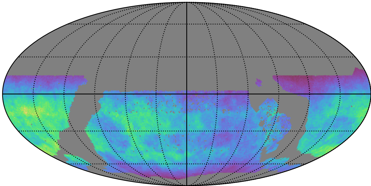
too_5_4v3.4_10yrs WFD u band: Normalized Teff
