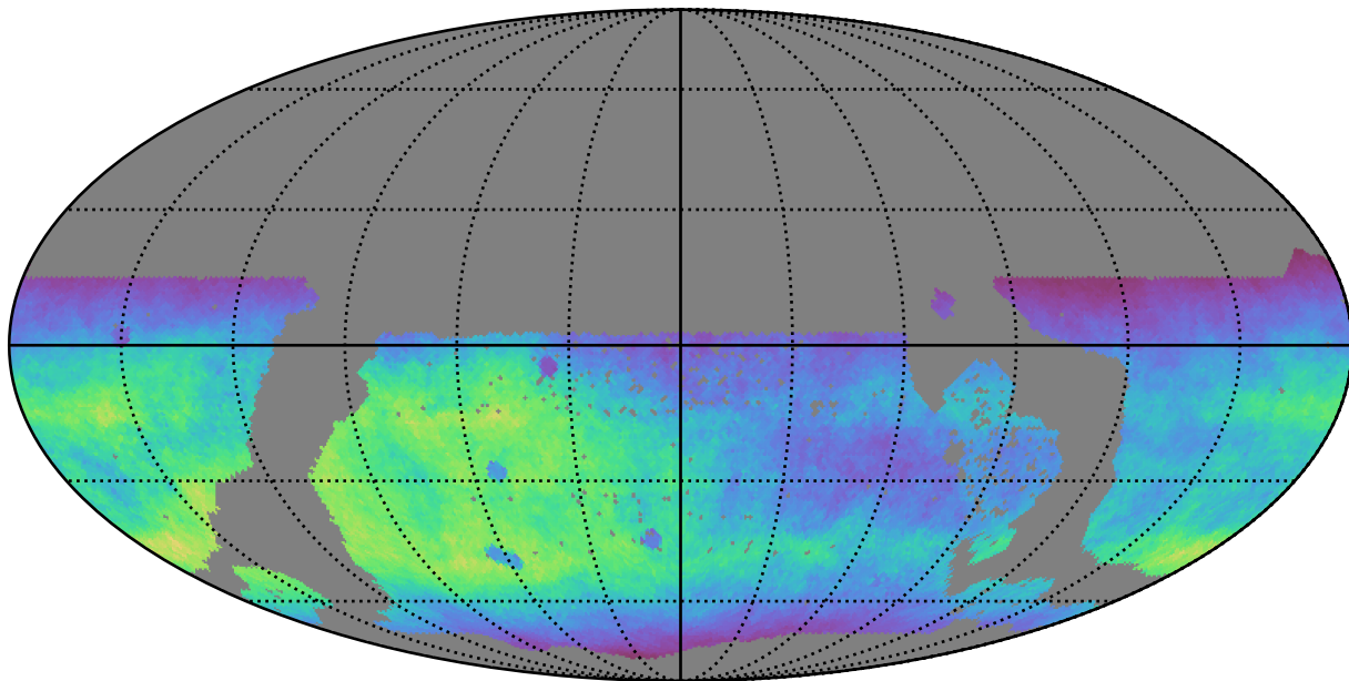
too_5_4v3.4_10yrs WFD r band: Normalized Teff
