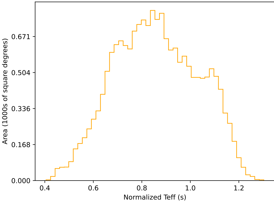
too_5_4v3.4_10yrs WFD r band: Normalized Teff
