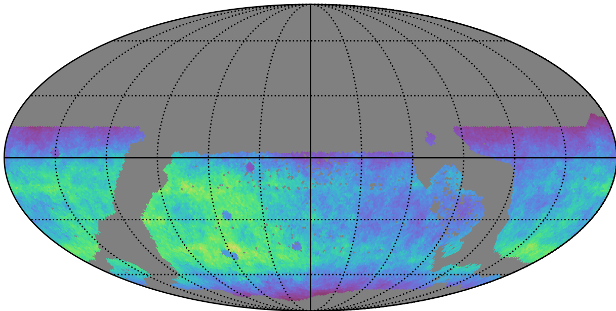
too_5_4v3.4_10yrs WFD g band: Normalized Teff
