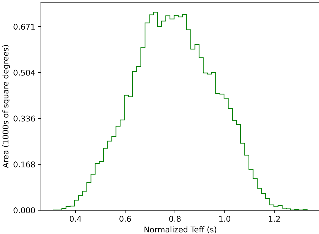
too_5_4v3.4_10yrs WFD g band: Normalized Teff
