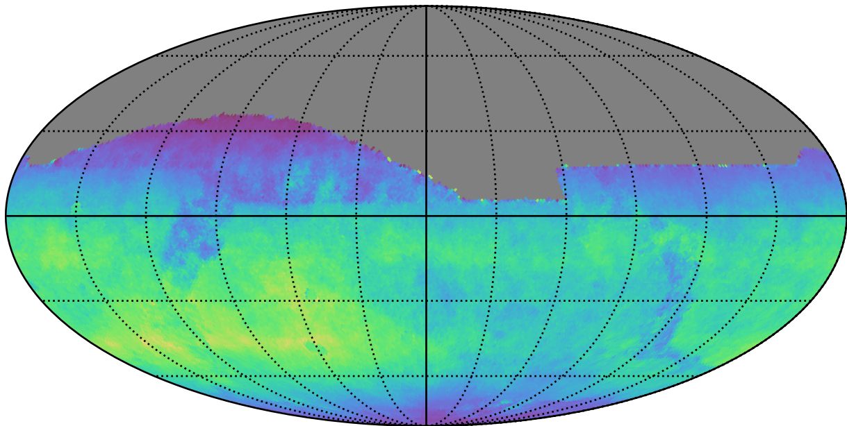
too_5_4v3.4_10yrs All sky z band: Normalized Teff
