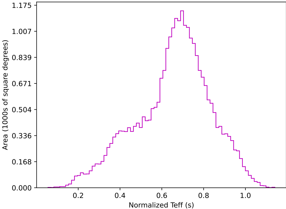
too_5_4v3.4_10yrs All sky z band: Normalized Teff
