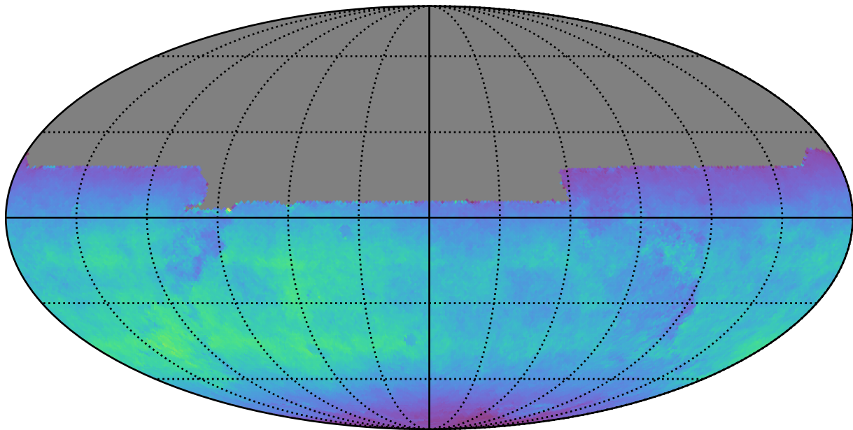
too_5_4v3.4_10yrs All sky y band: Normalized Teff
