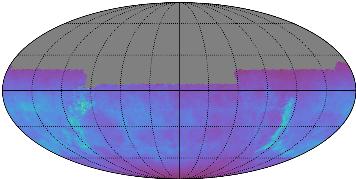
too_5_4v3.4_10yrs All sky u band: Normalized Teff
