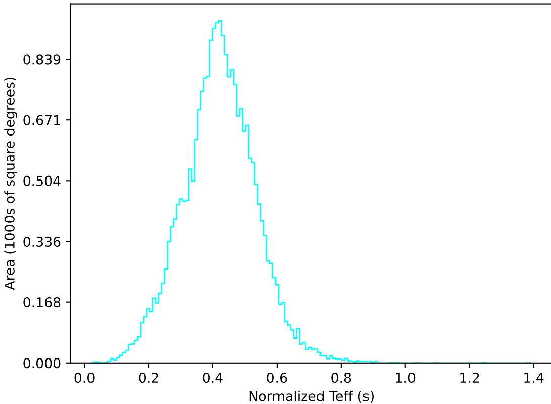
too_5_4v3.4_10yrs All sky u band: Normalized Teff
