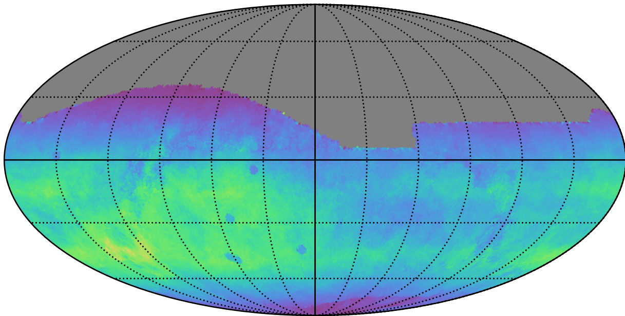
too_5_4v3.4_10yrs All sky r band: Normalized Teff
