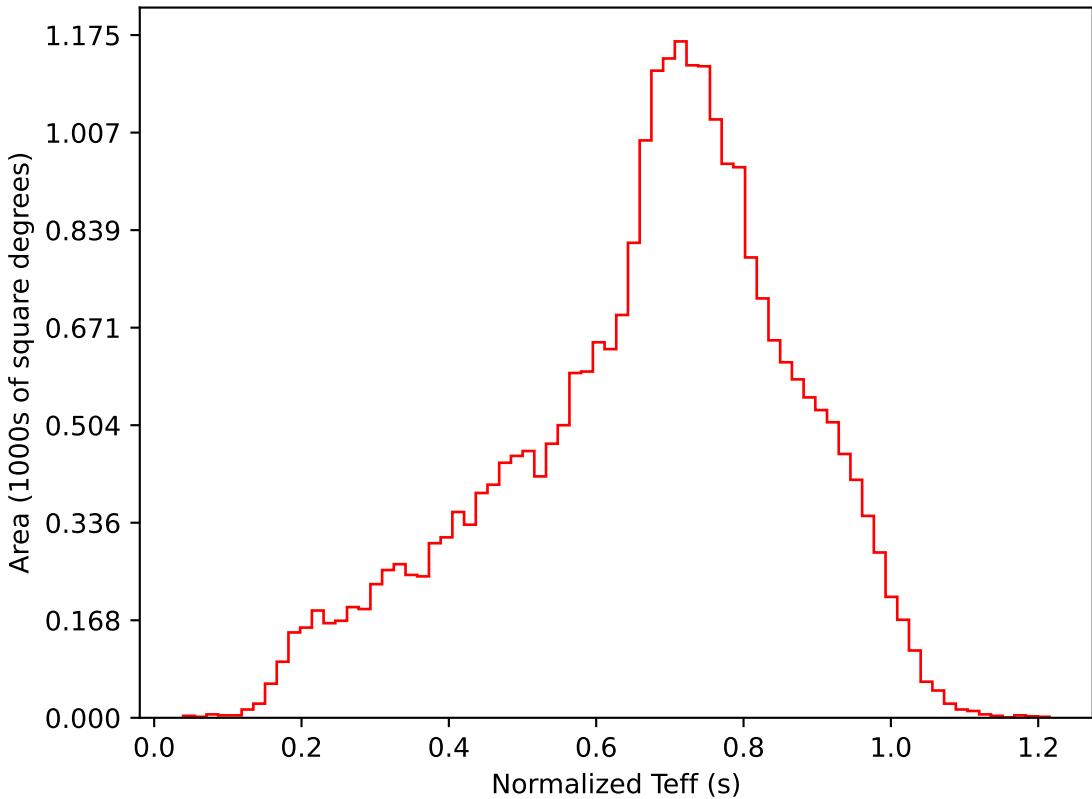
too_5_4v3.4_10yrs All sky i band: Normalized Teff
