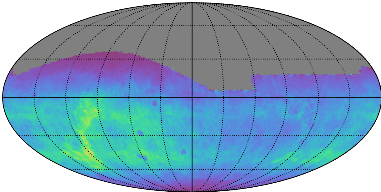
too_5_4v3.4_10yrs All sky g band: Normalized Teff
