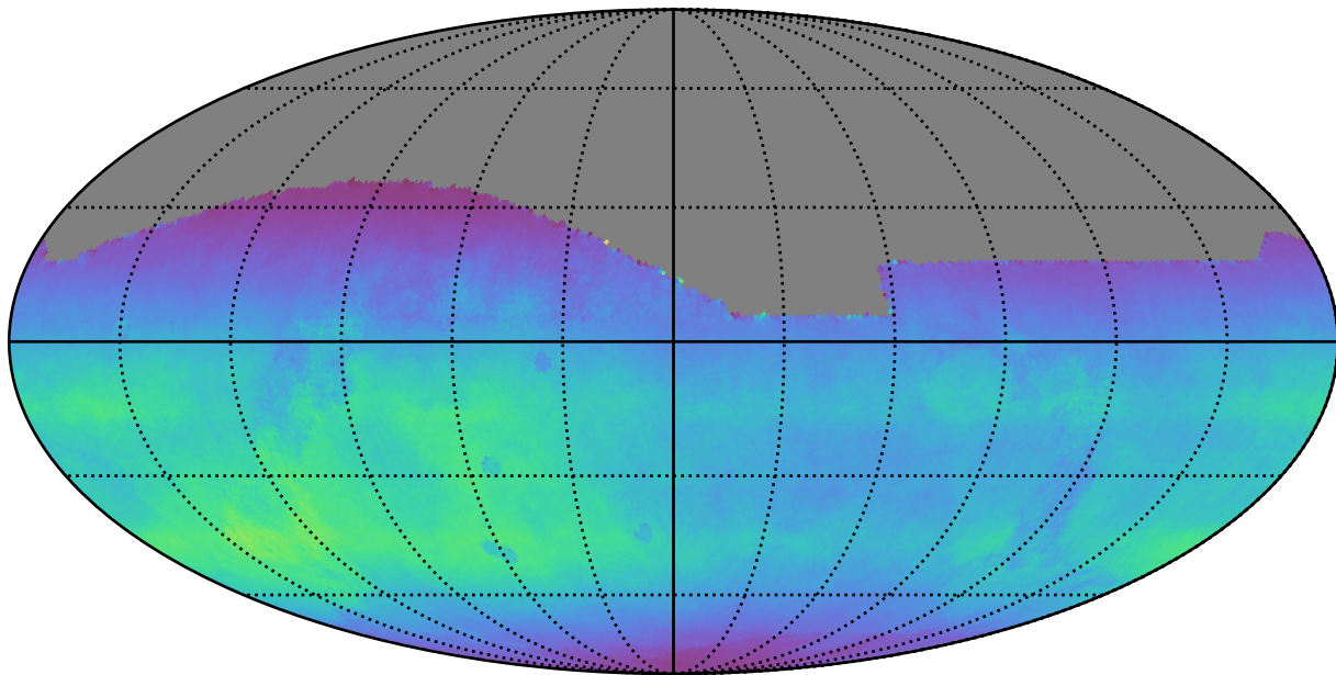
too_5_4v3.4_10yrs All sky all bands: Normalized Teff
