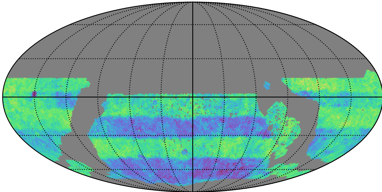
too_5_4v3.4_10yrs WFD: Normalized Proper Motion Uncert @ 24.0
