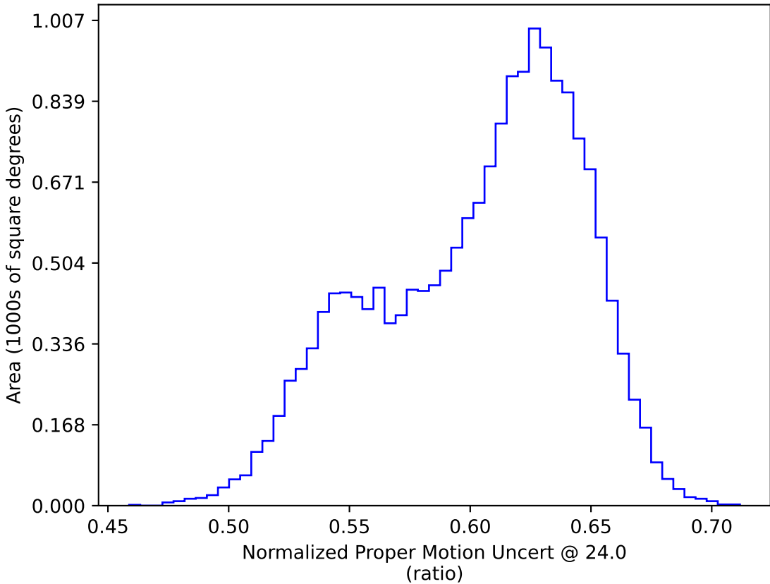
too_5_4v3.4_10yrs WFD: Normalized Proper Motion Uncert @ 24.0
