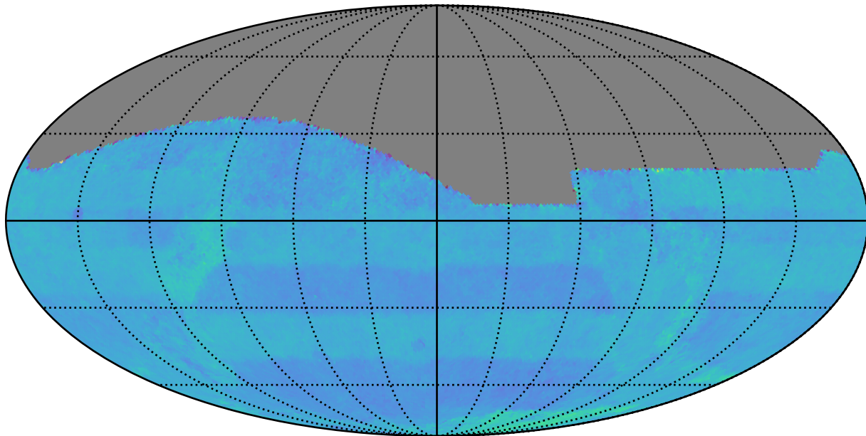
too_5_4v3.4_10yrs All sky: Normalized Proper Motion Uncert @ 24.0
