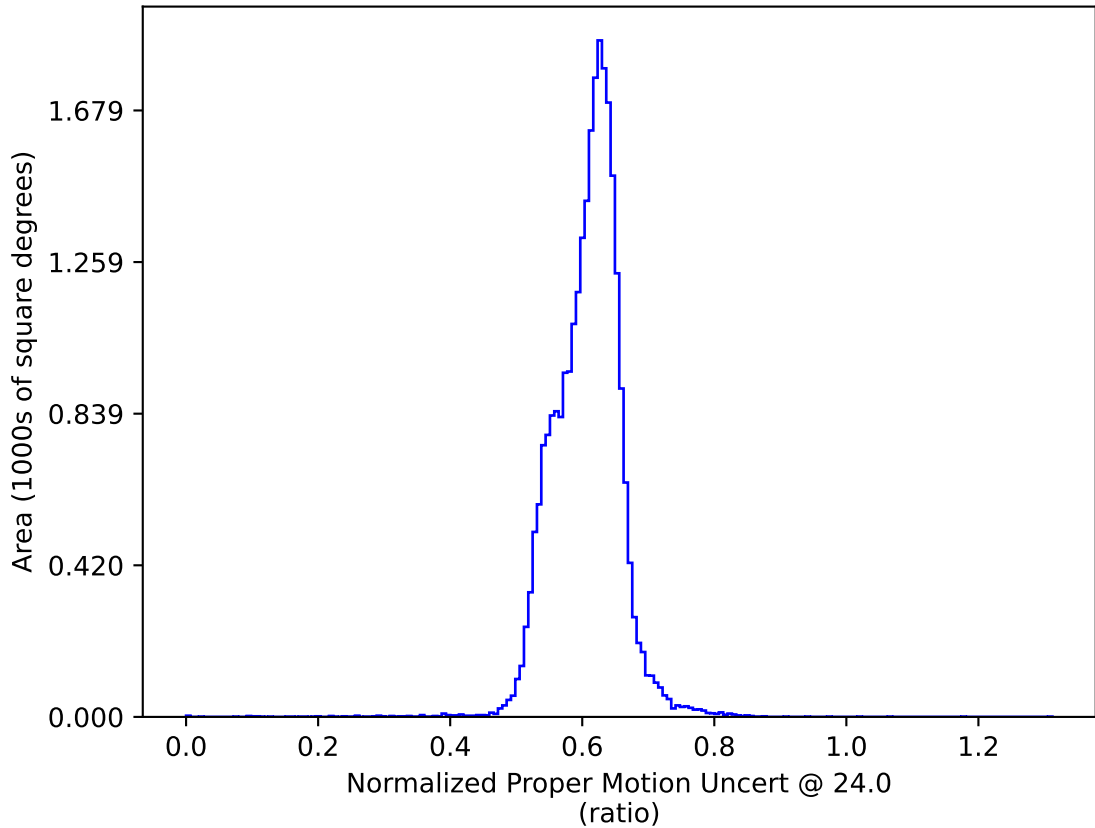
too_5_4v3.4_10yrs All sky: Normalized Proper Motion Uncert @ 24.0
