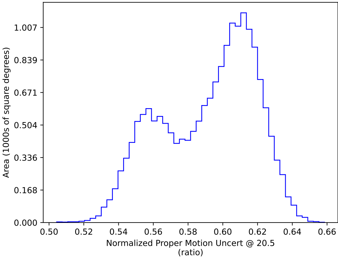
too_5_4v3.4_10yrs WFD: Normalized Proper Motion Uncert @ 20.5
