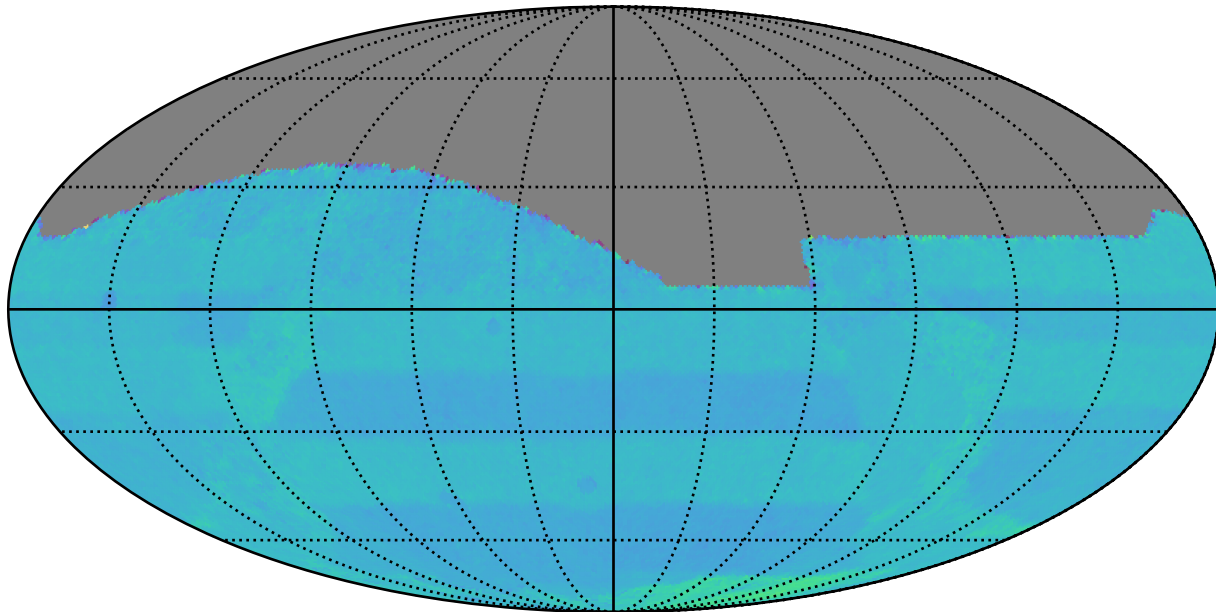
too_5_4v3.4_10yrs All sky: Normalized Proper Motion Uncert @ 20.5
