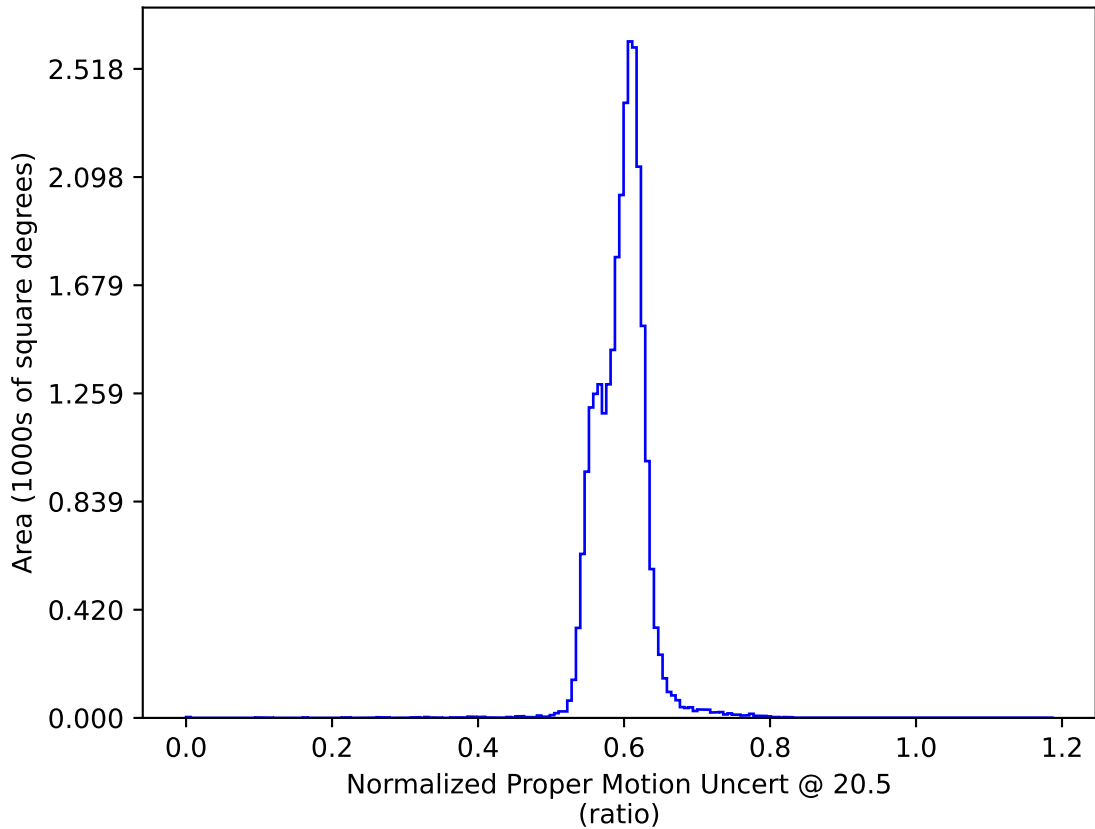
too_5_4v3.4_10yrs All sky: Normalized Proper Motion Uncert @ 20.5
