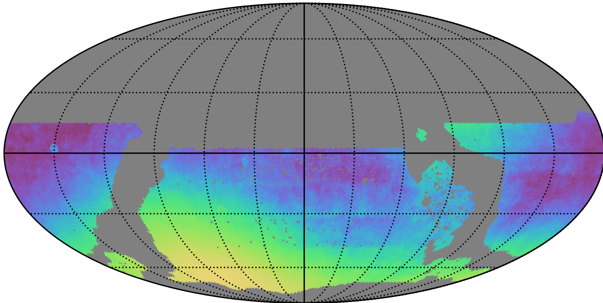
too_5_4v3.4_10yrs WFD: Normalized Parallax Uncert @ 24.0
