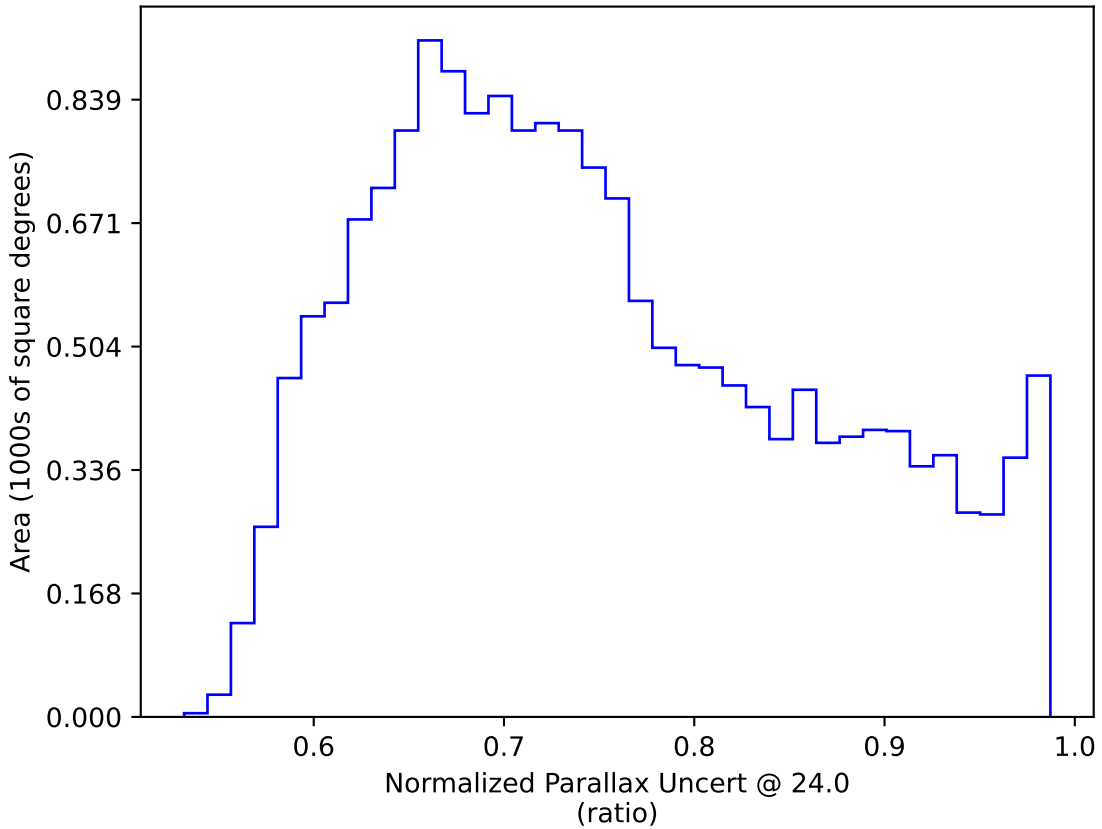
too_5_4v3.4_10yrs WFD: Normalized Parallax Uncert @ 24.0
