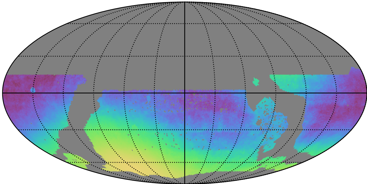
too_5_4v3.4_10yrs WFD: Normalized Parallax Uncert @ 22.4
